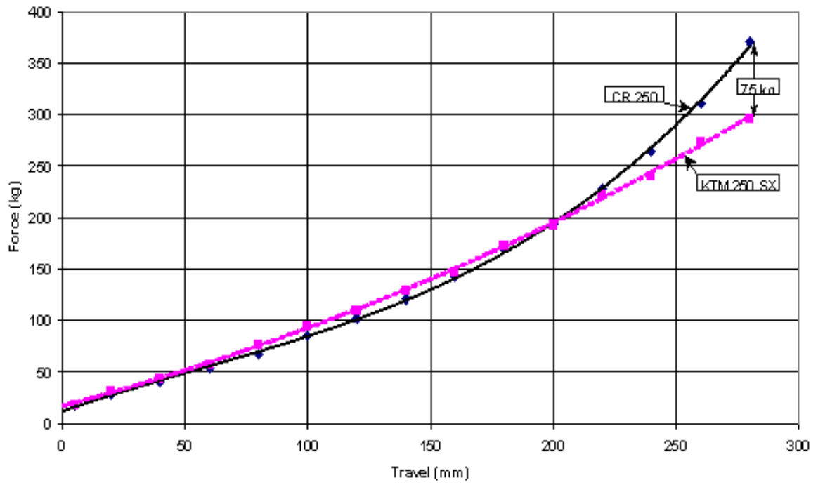
Rear Wheel Force Comparison 02 CR 250 vs. 02 KTM SX 250
